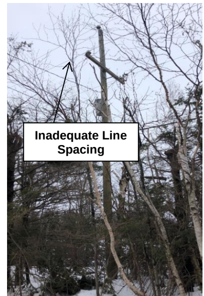
Figure 4 Structures with inadequate line spacing that do not meet current standards.
