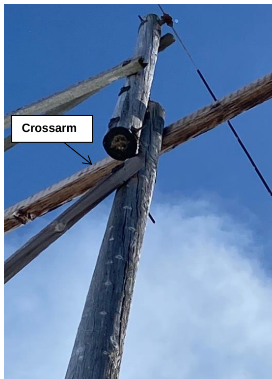
Rotten crossarm.
