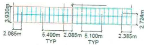
DETAIL-CONDITION B: 2x13 TABLE BESIDE 2x13 TABLE SCALE NTS
